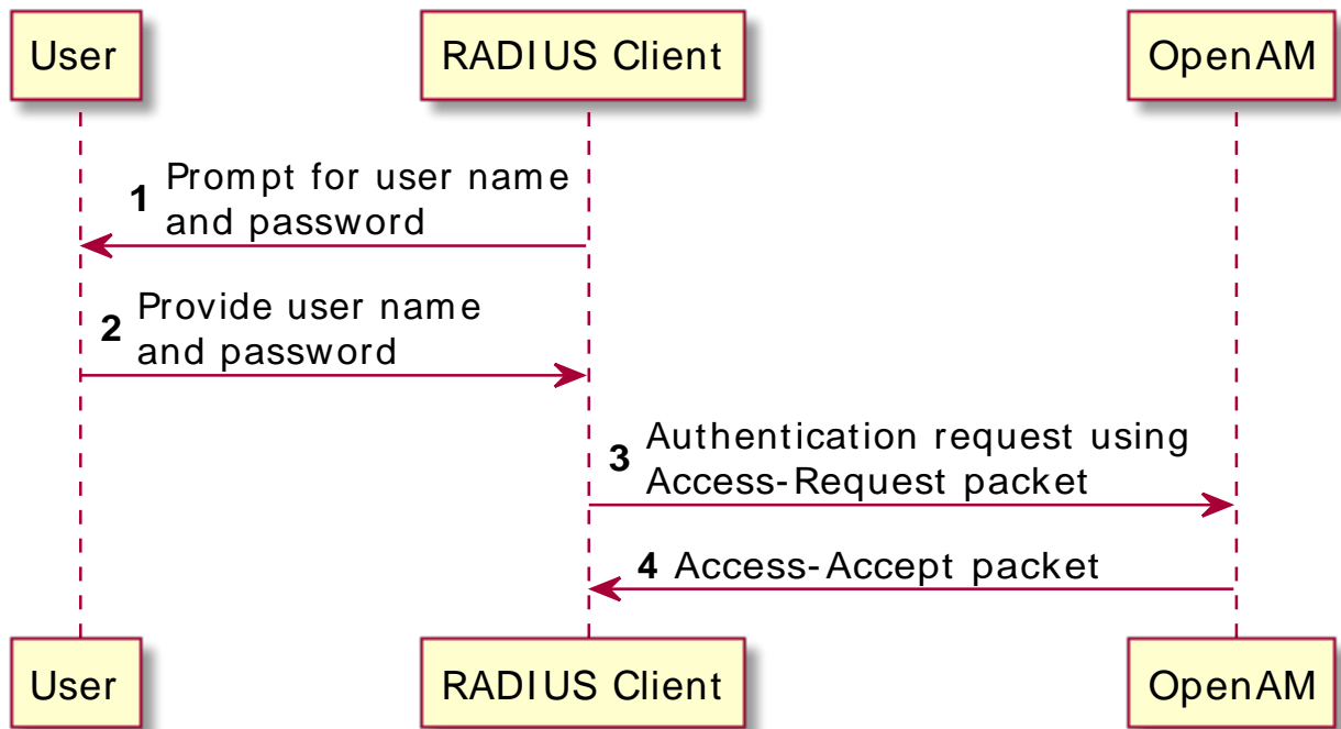
Figure 1.2. RADIUS Server Service: Successful Simple Authentication Flow
