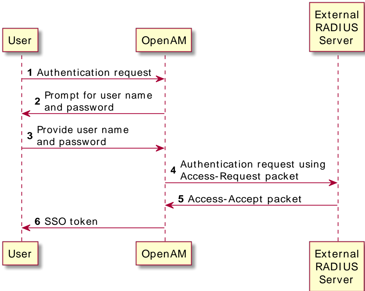
Figure 1.1. RADIUS Authentication Module: Successful Authentication Flow
