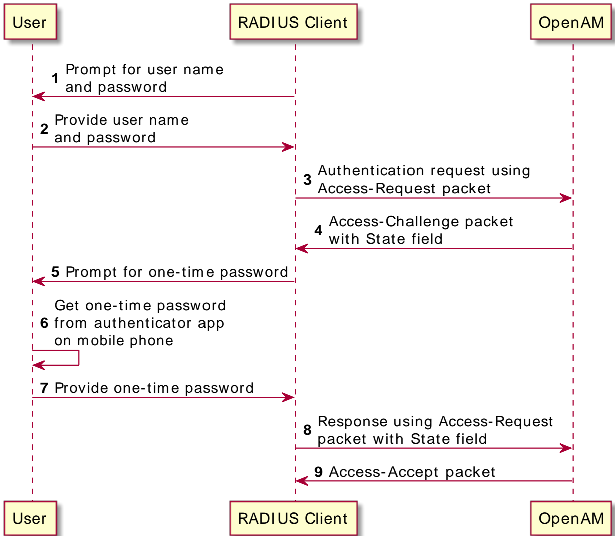
Figure 1.3. RADIUS Server Service: Successful Multi-Factor Authentication Flow
