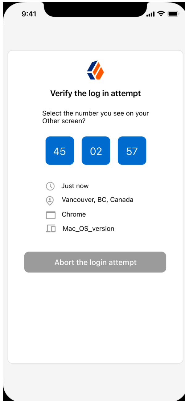
Figure 3. Challenge code
