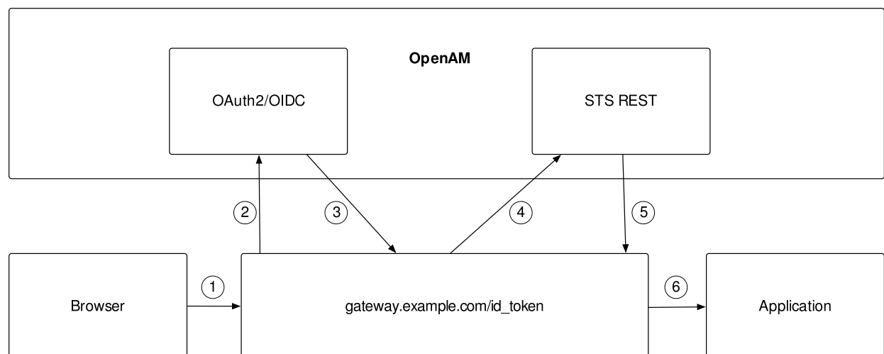
Figure 6. Token Transformation
