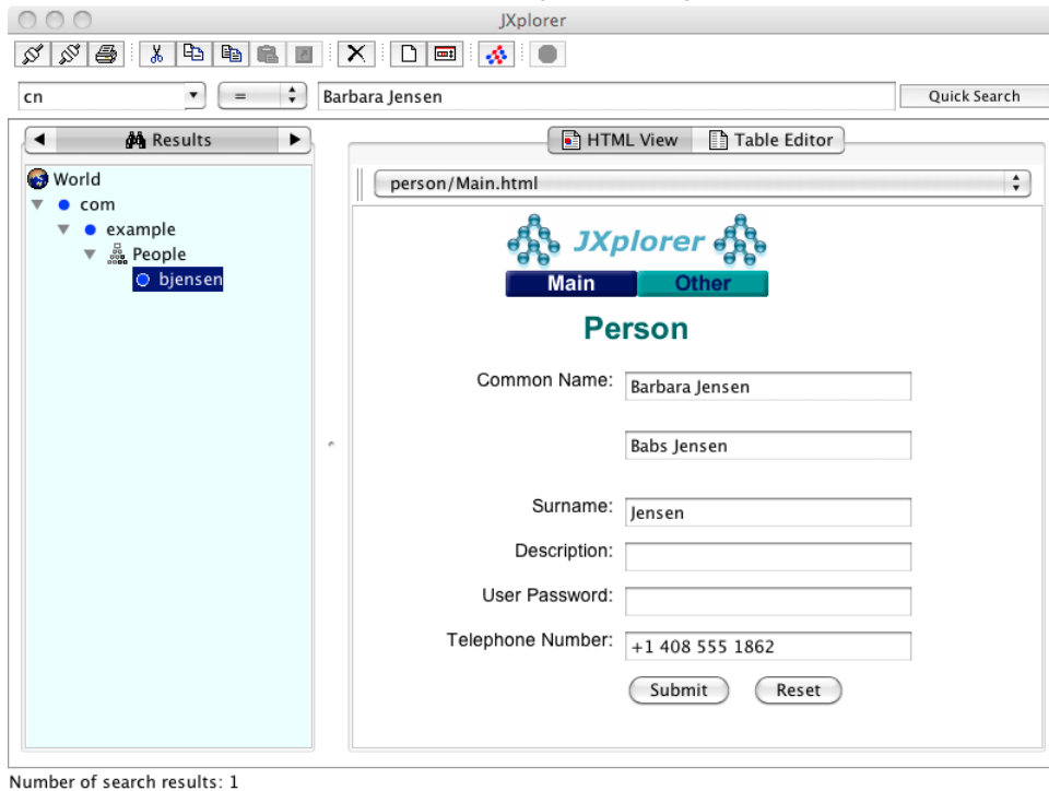
JXplorer accessing OpenDJ through DSML
